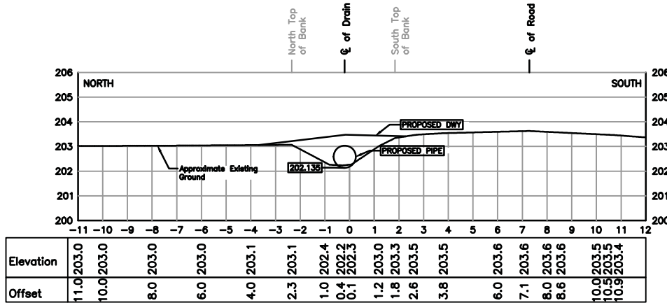
CL OF PROPOSED BRIDGE-STA. 0+742.45 Scale=1:100
