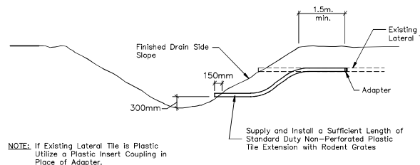
STANDARD LATERAL TILE DETAIL
