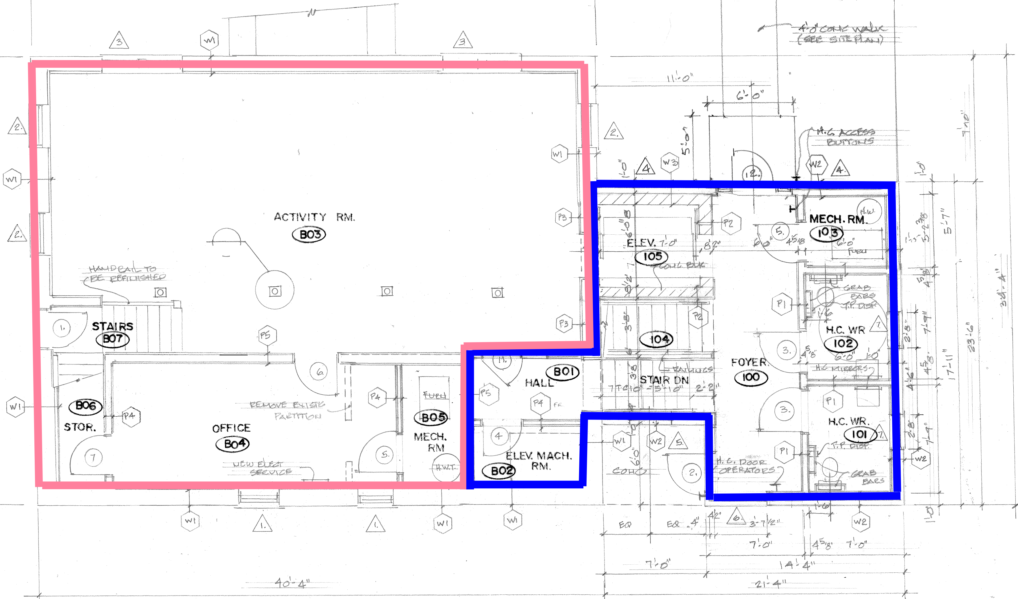
MAIN FLOOR & BASEMENT FLOOR PLAN
